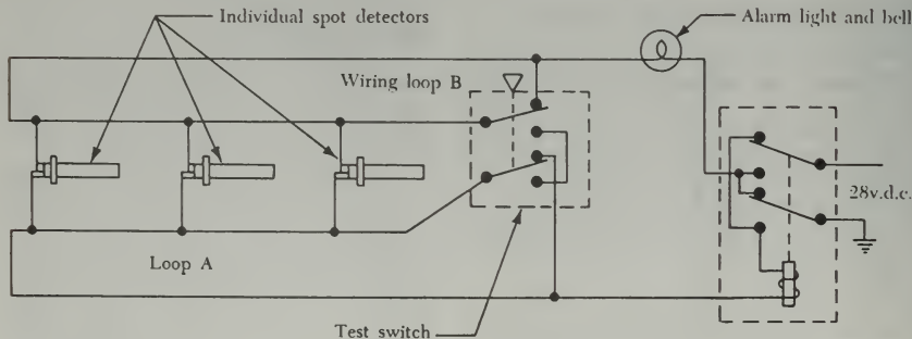
FIGURE 9-6. Fenwal spot-detector circuit.
